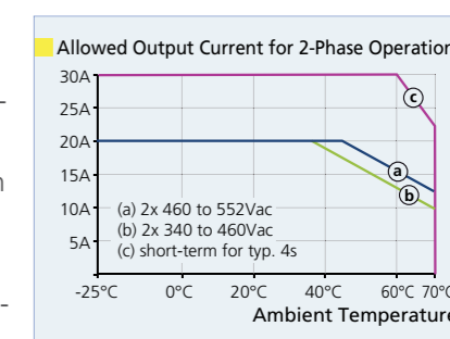
Allowed output power for 2-phase operation (example: QT20.241)
