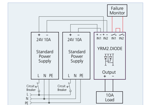
Wiring scheme of a 10A redundant system with the redundancy module YRM2.DIODE
