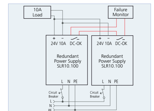
Wiring scheme of a 10A redundant system with two redundant power supplies SLR10.100
